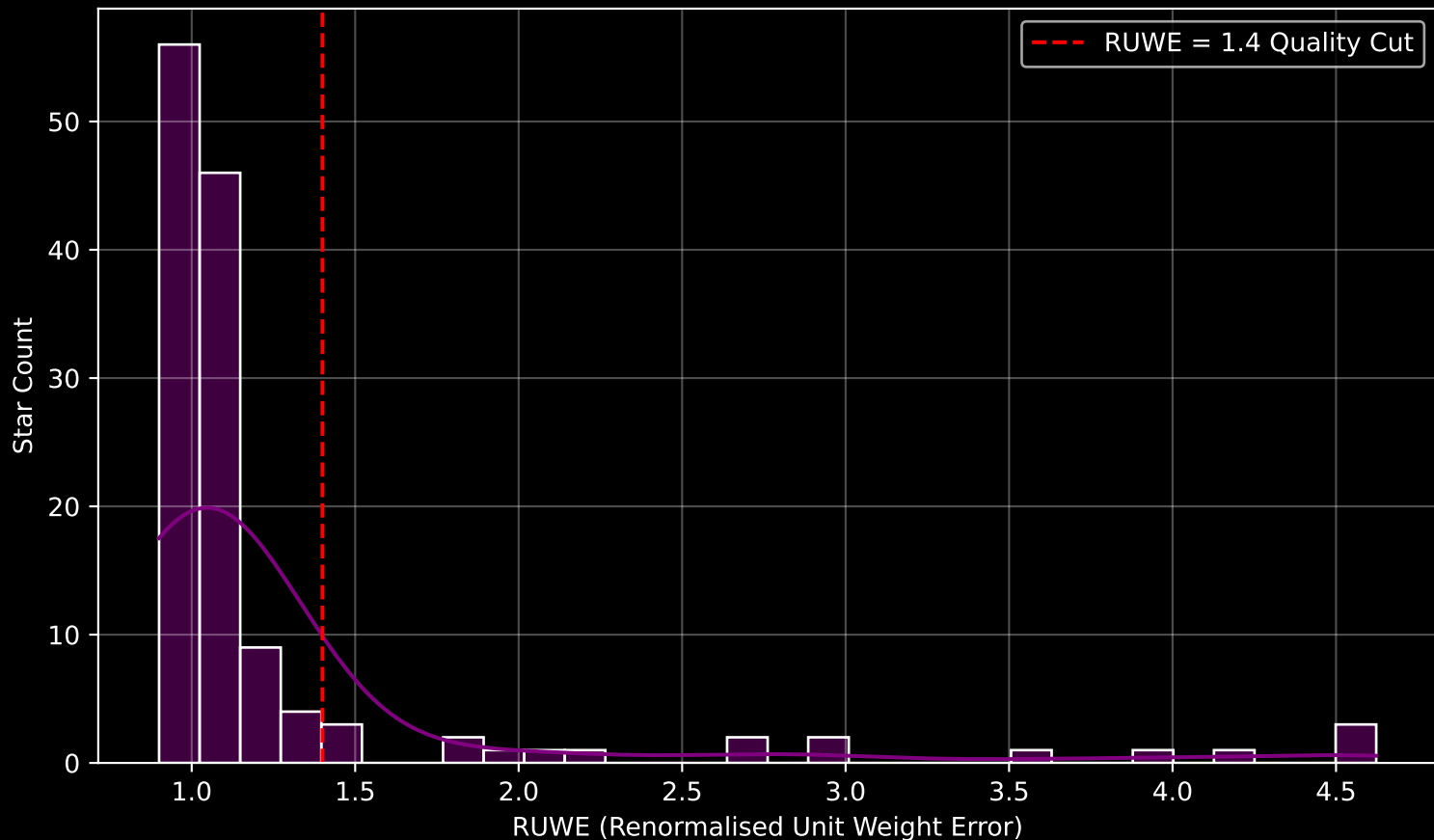
GAPOGEE DR17 Field [ORIOND] RUWE Distribution (n= 133)
