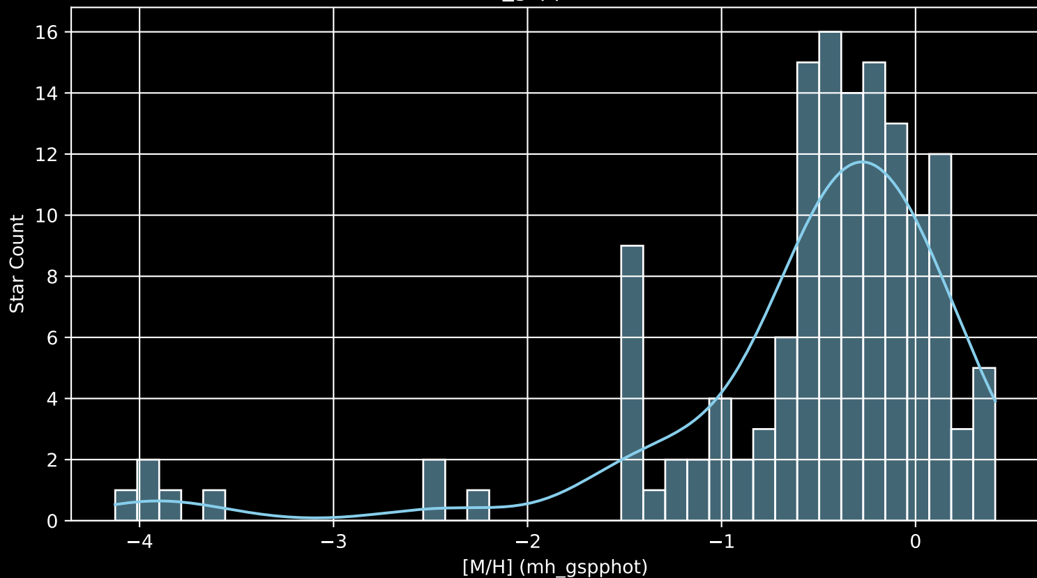
APOGEE DR17 Field: [ORIOND [M/H] (mh_gspphot) (n= 140)
