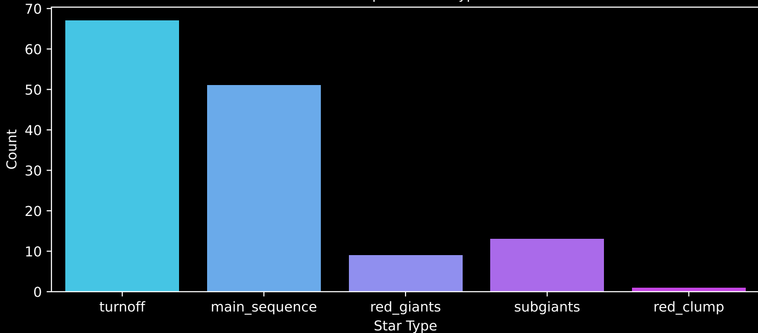
APOGEE DR17 Field: [ORIOND] Count plot of Star Type
