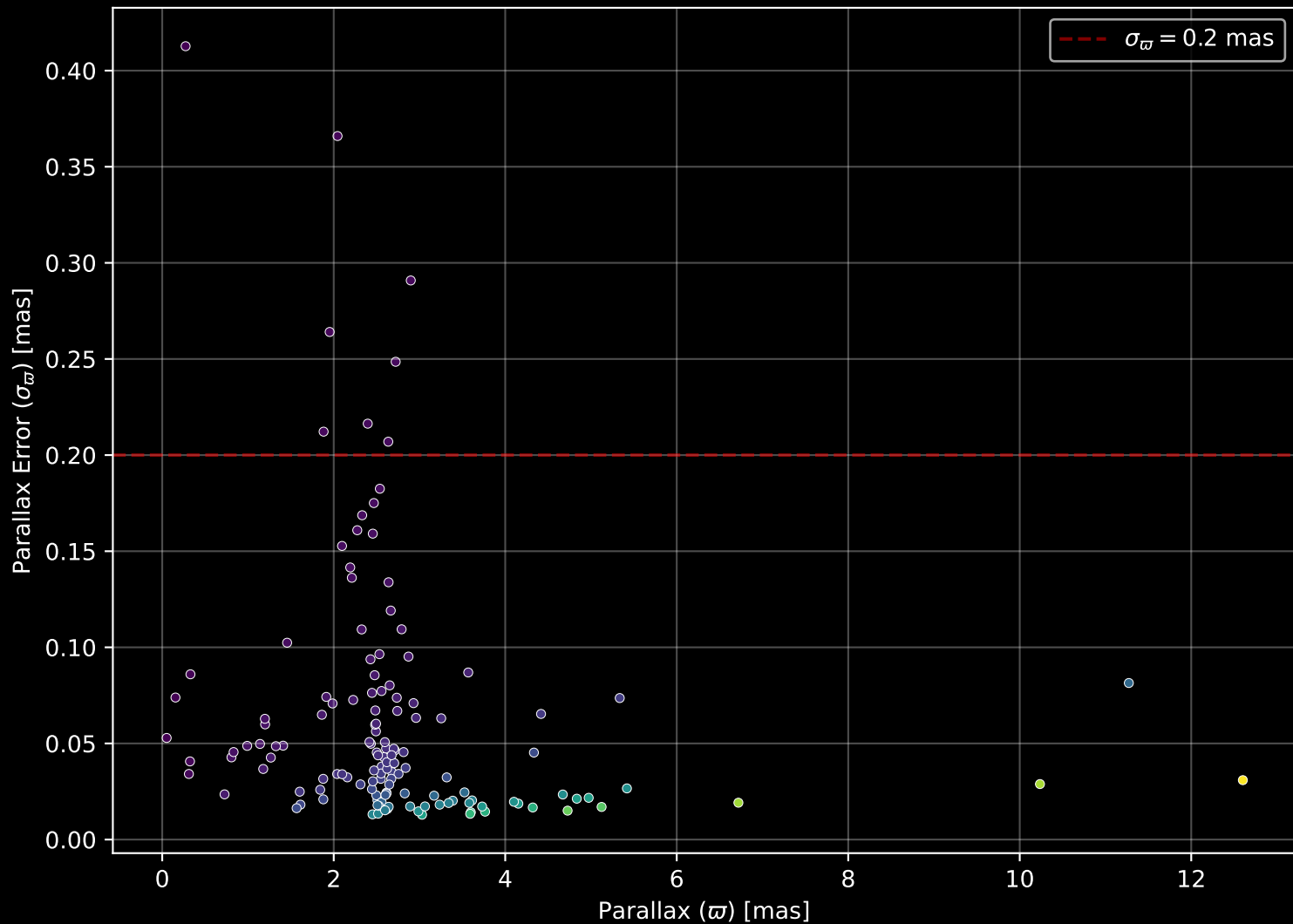
APOGEE DR17 Field: [ORIOND] Parallax Quality (n= 141)
