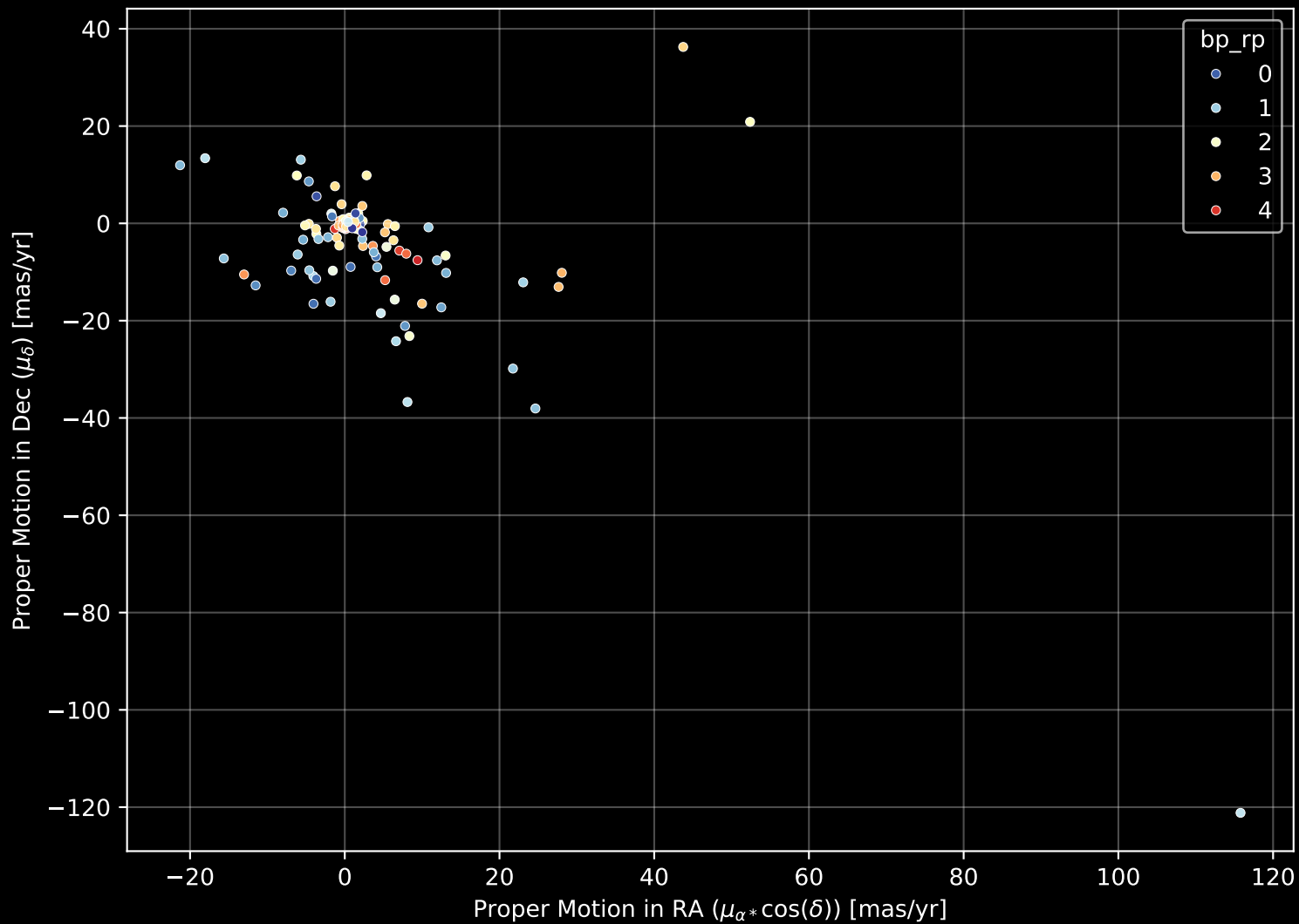
APOGEE DR17 Field: [ORIOND] Proper Motion Diagram (n= 141)
